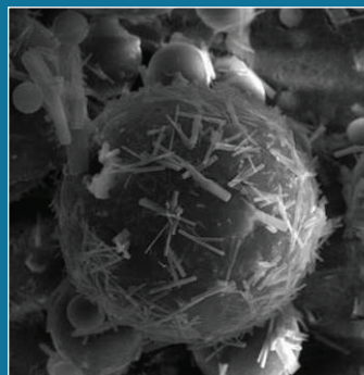
Deltamethrin crystals forming at interface of carrier and aqueous solution
