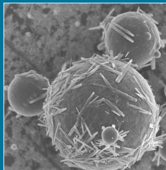
Deltamethrin crystals forming at interface of carrier and aqueous solution
