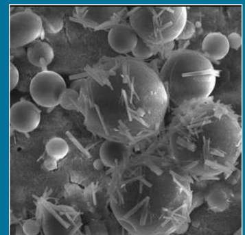
Deltamethrin crystals forming at interface of carrier and aqueous solution
